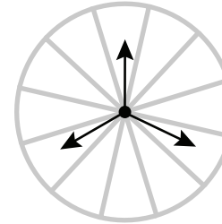
3 COLORS TRIADIC
